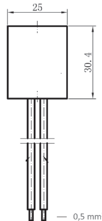
Bistabile Spulen (SQ-A27/D27 Series)
